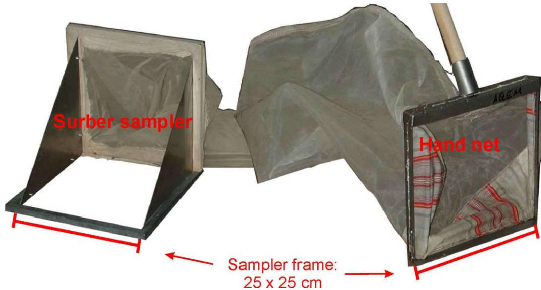
Figure 33: Surber sampler and hand-net
