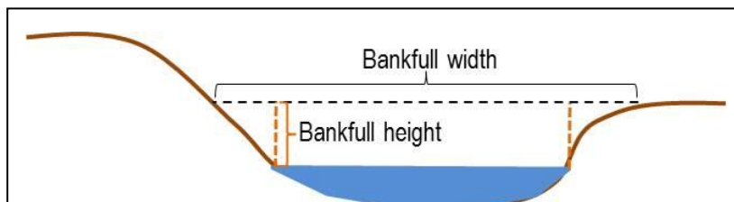
Figure 29: Example for determining bankfull discharge and measuring the height of left/right bank at a transect.
