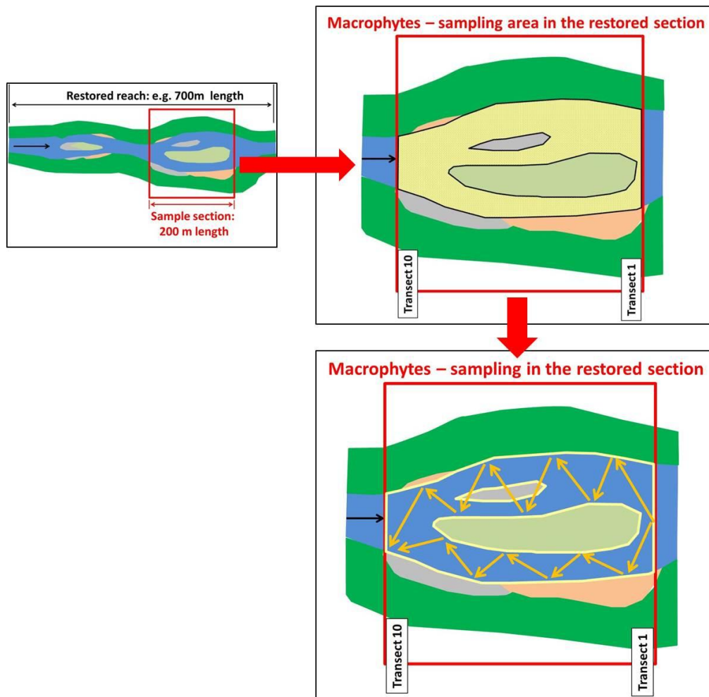
Figure 42: Sampling of macrophytes in the restored section (sample area is marked in yellow; orange arrows show the way of wading)
