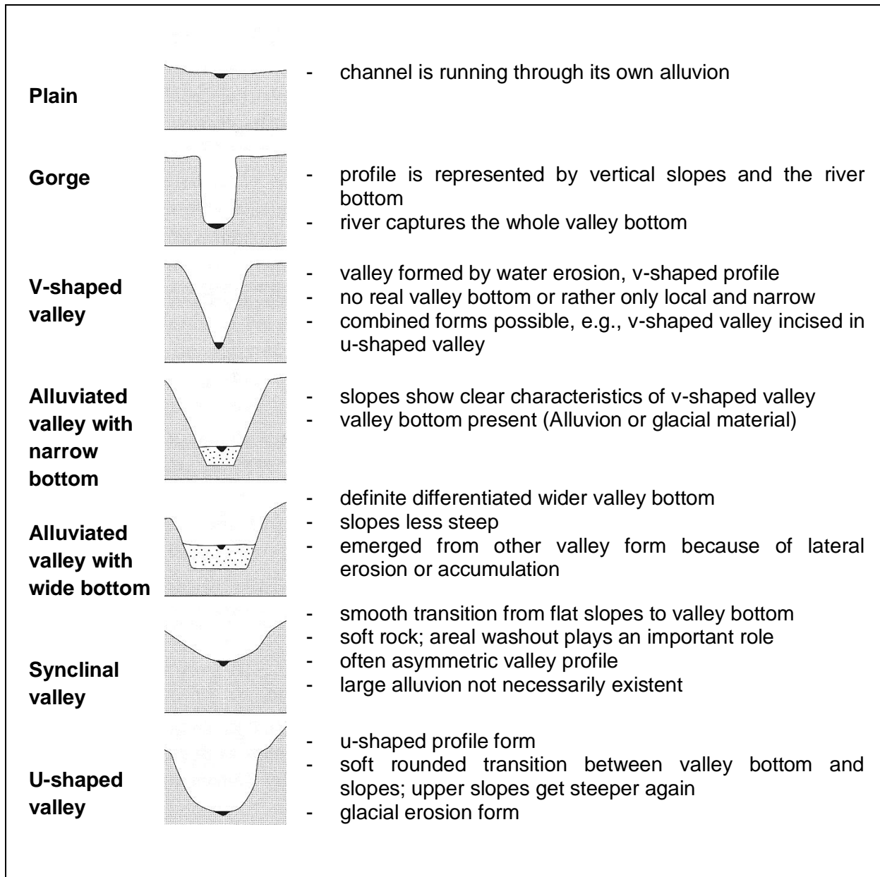
Figure 10: Valley types (Muhar et al. 2000, Jungwirth et al. 2003 based on Mangelsdorf et al. 1990)
