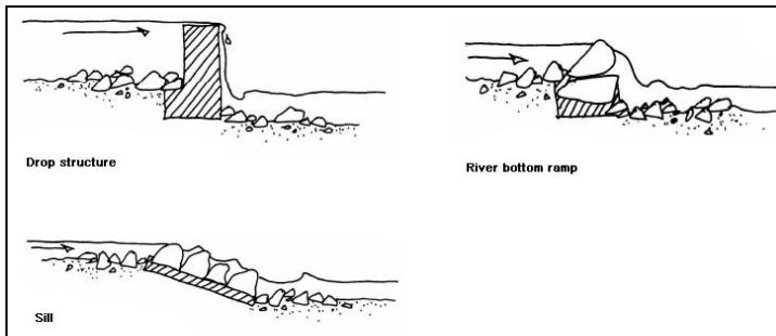
Figure 8: Examples for structures interrupting the river continuum (freiland Umweltconsulting 2001)
