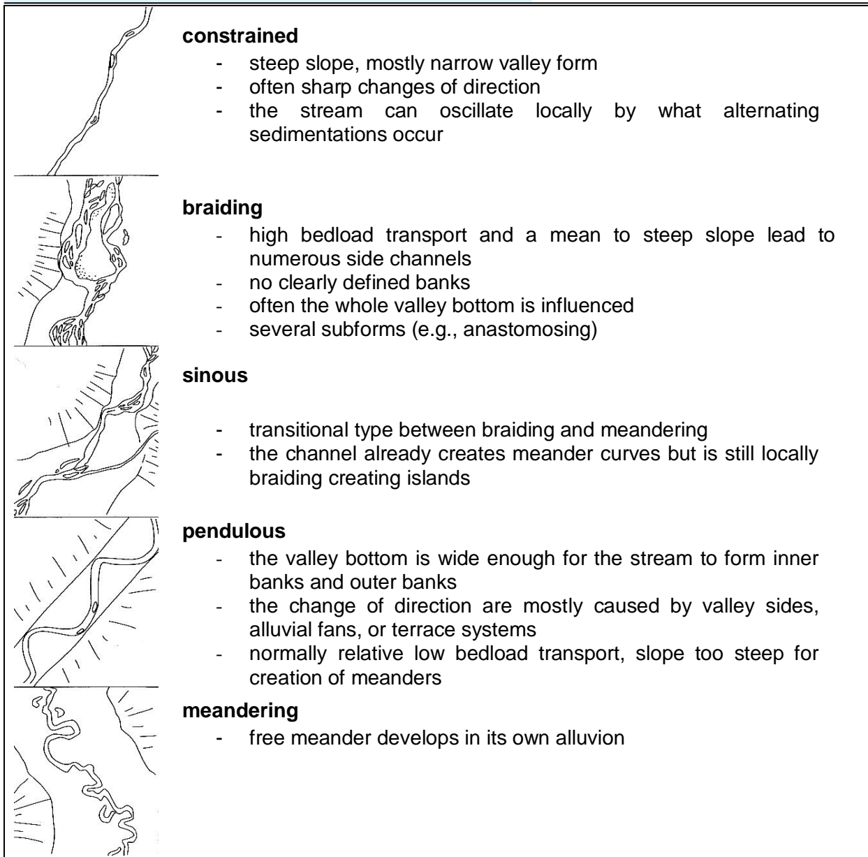
Figure 11: Morphological River Types (Muhar et al. 2000, Jungwirth et al. 2003)
