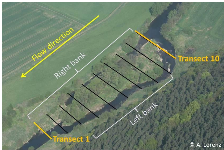
Figure 28: Example of a sample section with ten transects (black lines) for mapping of hydromorphology
