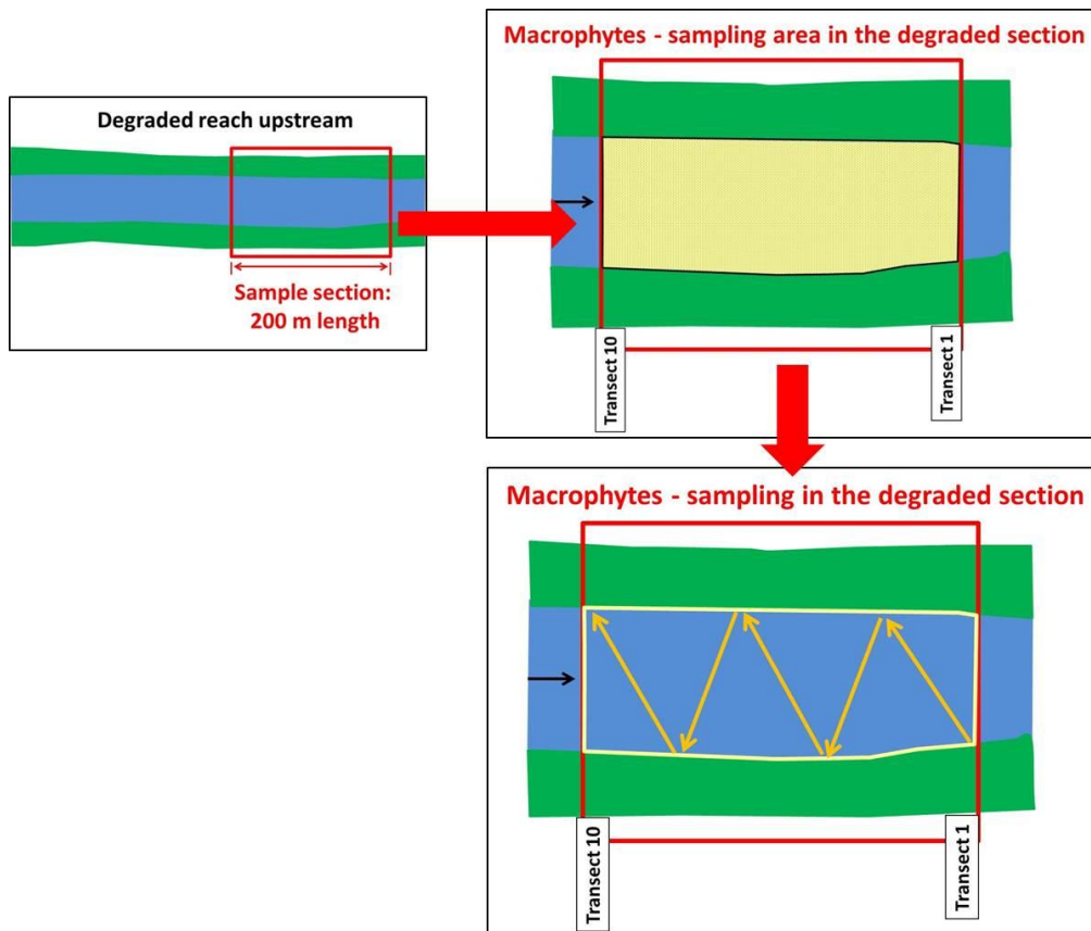
Figure 41: Sampling of macrophytes in the degraded section (sample area is marked in yellow; orange arrows show the way of wading)
