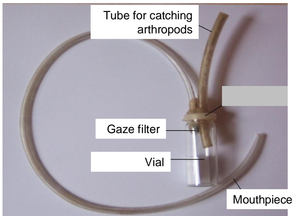
Figure 47: Exhaustor
